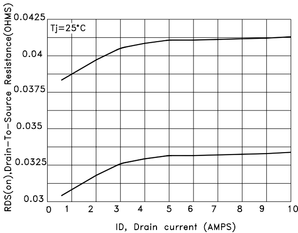
Fig.4 On-Resistance versus Drain Current and Gate V0
